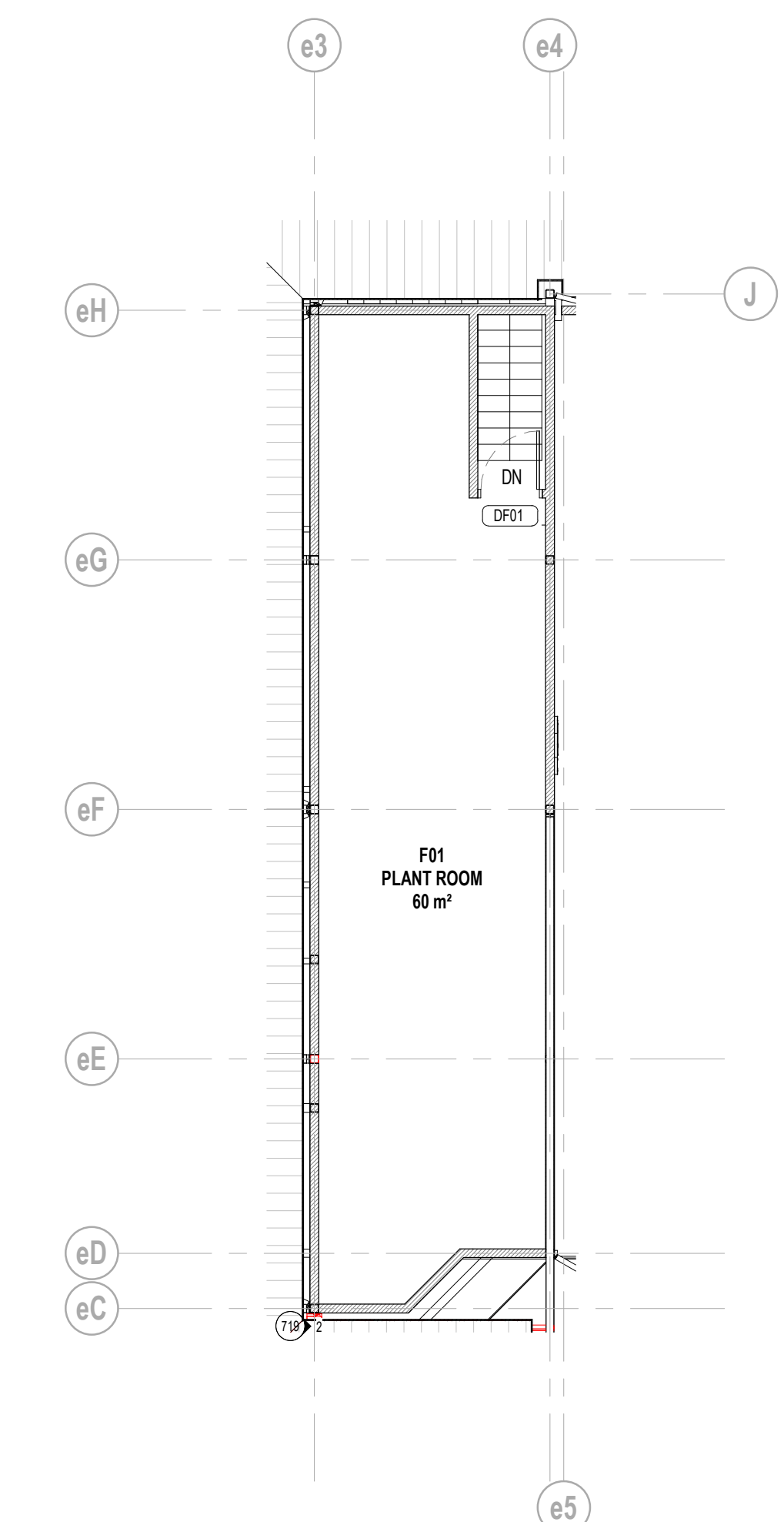
PROPOSED FIRST FLOOR PLAN 1:100
